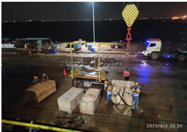
Loading operations (Box cargo)
