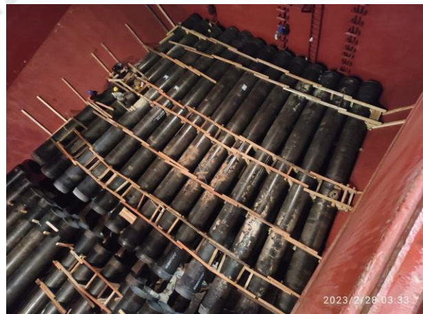
Hold №4 Cargo position
