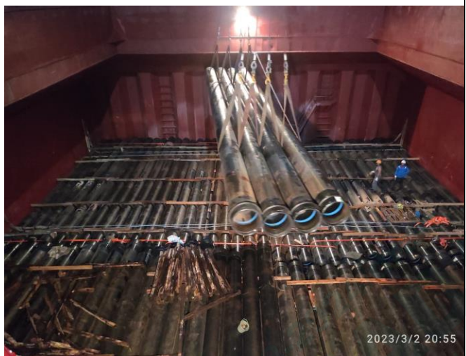
Hold № 2 Loading operations
