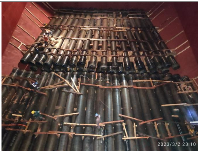
Hold №4 Dunnage preparation
