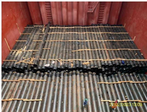
Hold №2 Cargo position
